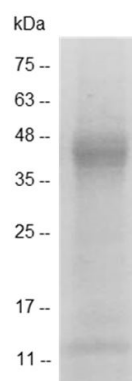
SDS-PAGE analysis of recombinant human HMGB1
