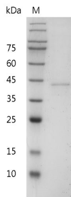
SDS-PAGE analysis of recombinant mouse IL-12 p40
