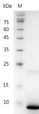
SDS-PAGE analysis of recombinant human CXCL3
