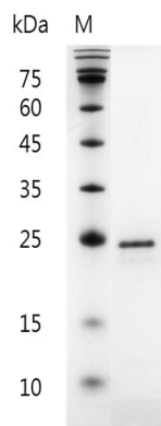
SDS-PAGE analysis of recombinant human FGF-20
